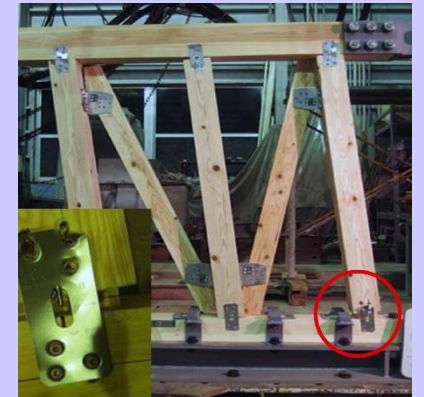
Experiment of wooden structure
